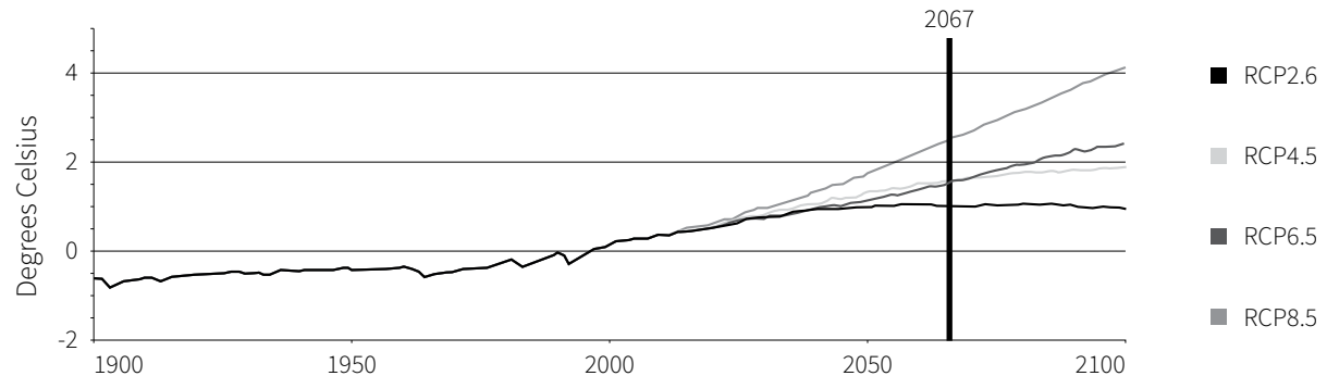
FIGURE 3 FORECASTED AVERAGE SURFACE TEMPERATURE CHANGE (RELATIVE TO 1986-2005), IPCC 2014
